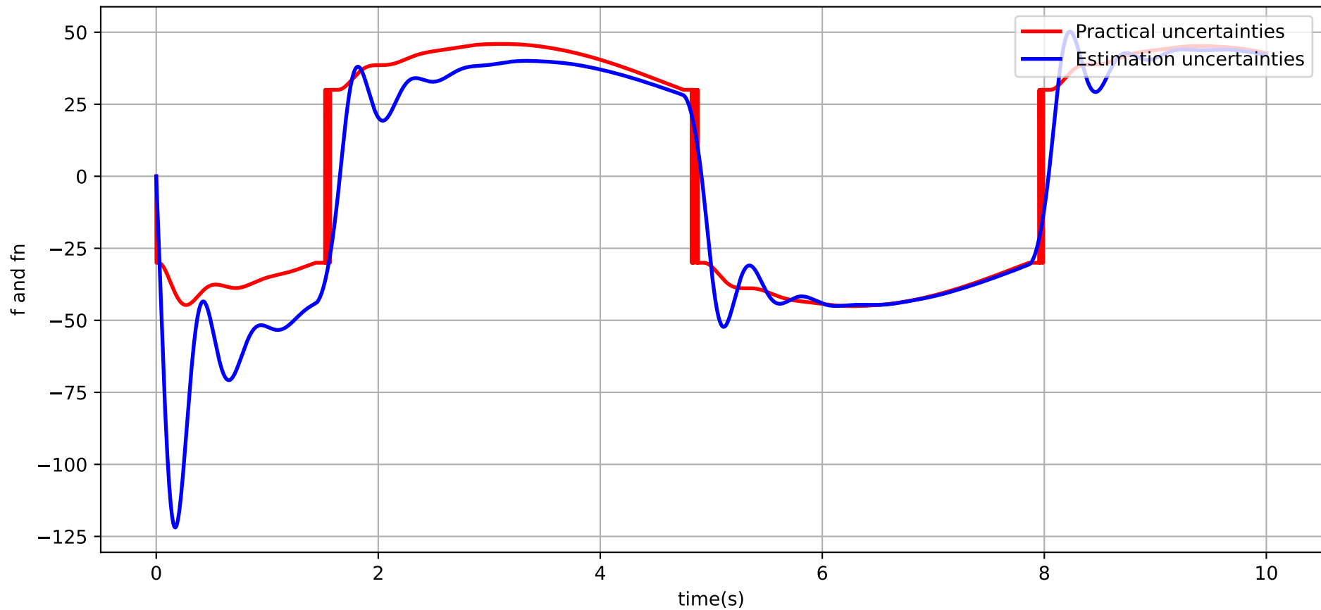
Disturbance Estimation Performance ( S=3 , S1=1 , m=19 )
